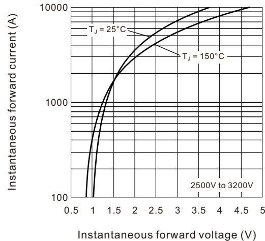
Fig.18 Forward voltage drop characteristics
